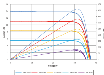
Current-Voltage & Power-Voltage Curve (420W)
