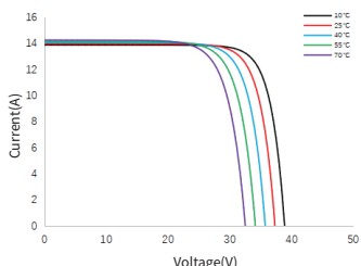
I-V Curve at Different Temperature SS8-54HSB -400M
