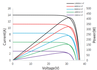
I-V/P-V Curve at Different Irradiation SS8-54HSB -400M
