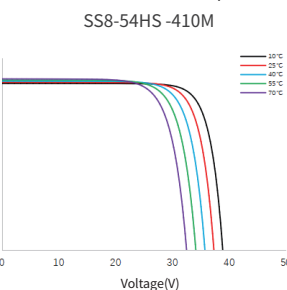
I-V Curve at Different Temperature
