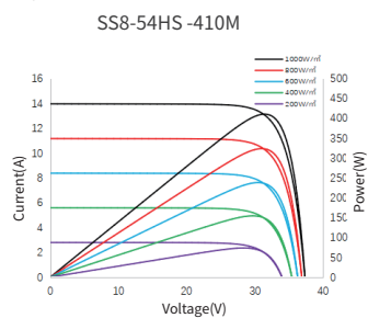
I-V/P-V Curve at Different Irradiation
