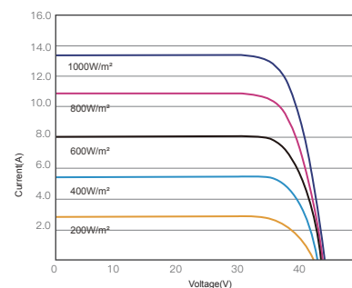
I-V CURVES OF PV MODULE(555W)
