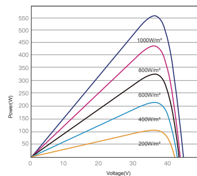
P-V CURVES OF PV MODULE(555W)
