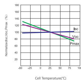
Power voltage current curve at different temperature
