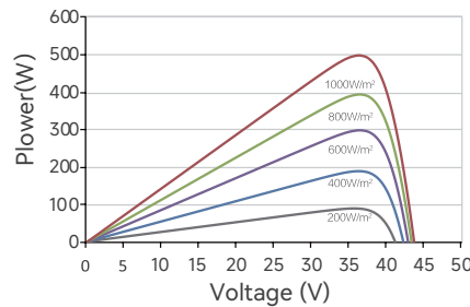
Power-Voltage(500W)
