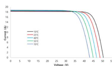
I-V Curve at Different Temperature SS9-66HD-710N
