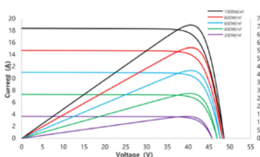
I-V/P-V Curve at Different Irradiation SS9-66HD-710N
