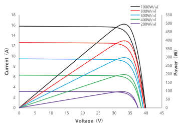
I-V/P-V Curve at Different Irradiation SSA-54HD-495N
