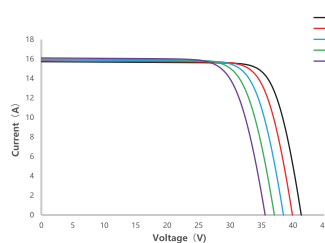
I-V Curve at Different Temperature SSA-54HD-495N
