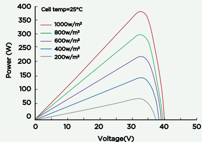
Power-Voltage Curve(400M-60H)
