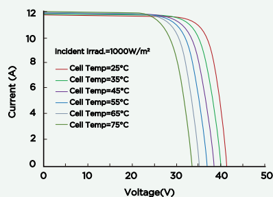
Current-Voltage Curve(400M-60H)
