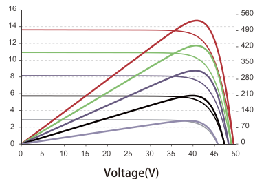
不同辐照度下电流电压曲线/功率电压曲线 (550W) Current voltage curve/power voltage curve under different irradiance(550W)
