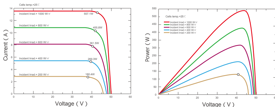
Current-Voltage & Power-Voltage Curves (RMH72-550S1)
