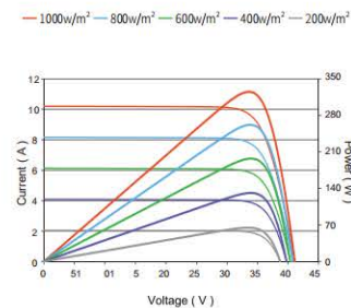
Current-Voltage & Power-Voltage Curves (330W)
