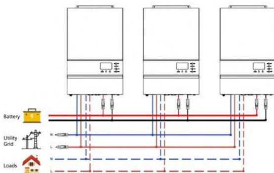
PARALLEL CONNECTION
