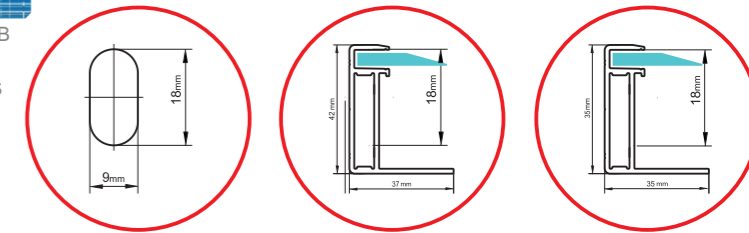
Mounting Slot
