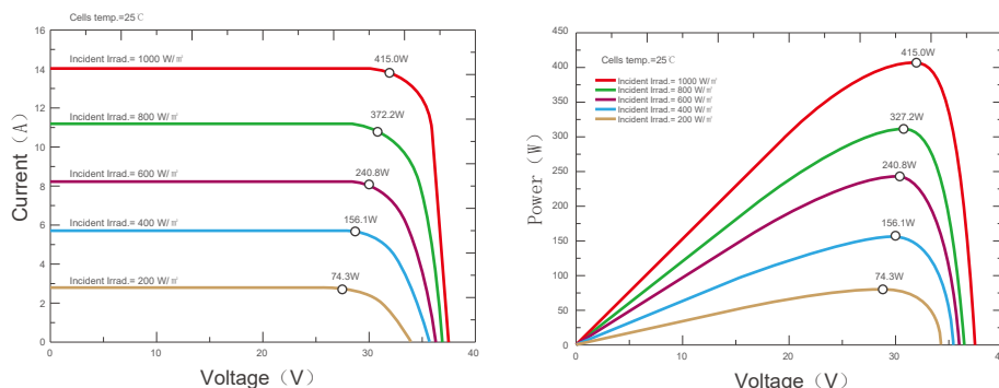
Current-Voltage & Power-Voltage Curves (RMH54-415S1)
