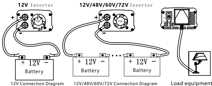
12V Connection Diagram
