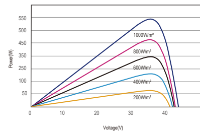
P-V Curves(550W)
