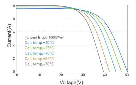
I-V curves of module under different temperature(350w)
