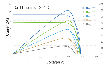
I-V curves/P-V curves of module under different irradiation(350w)
