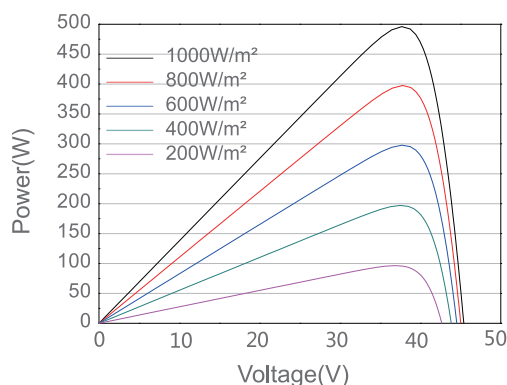
Power-Voltage Curve TP132-495M/MB-8
