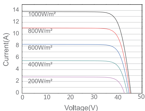
Current-Voltage Curve TP132-495M/MB-8
