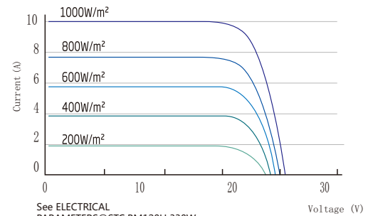
Current--Voltage
