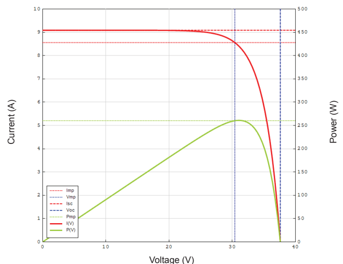
RNG-260D Characteristics Versus Voltage
