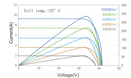
I-V curves/P-V curves of module under different irradiation(295w)
