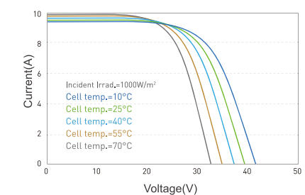
I-V curves of module under different temperature(295w)
