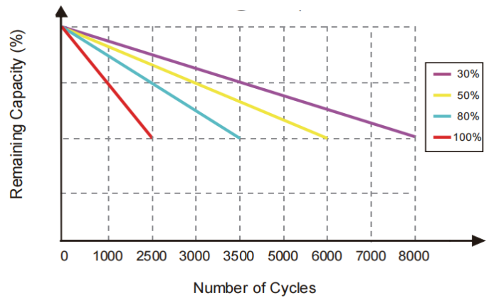
CYCLE LIFE vs. DEPTH OF DISCHARGE(DOD)
