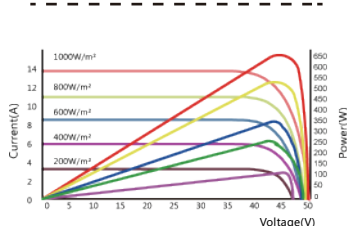
HS182-144M-530W
