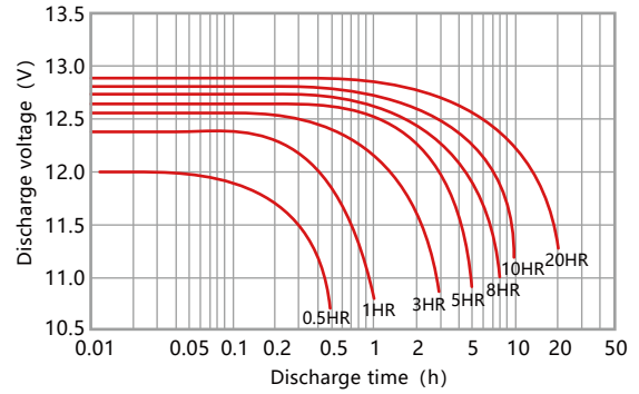
Discharge performance at different discharge rates (25°C/77°F)
