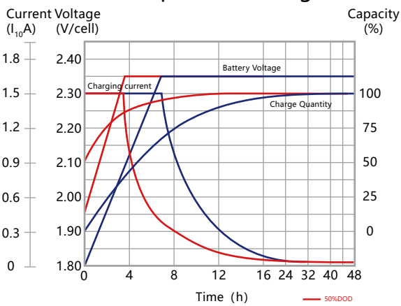
Constant-potential charge
