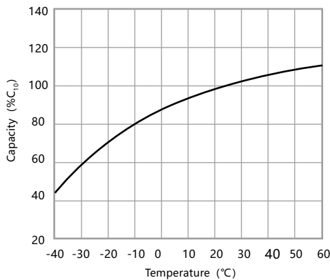
Temperature and discharge capacity
