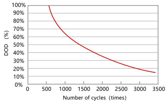
Cycle Service Life (25°C/77°F)
