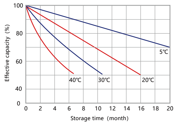
Self discharge parameters characteristics
