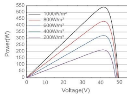
Power-Voltage Curve
