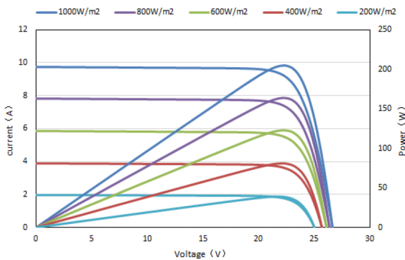
SEAC40T-205 I-V & P-V Curve
