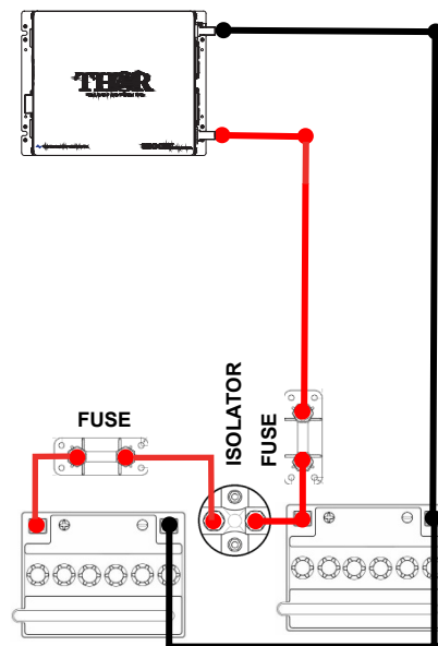
DUAL BATTERY INSTALLATION ISOLATING VEHICLE BATTERY
