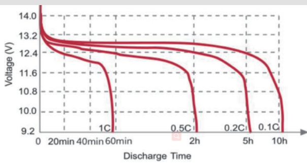
Different Rate Discharge Curve(25 °C)
