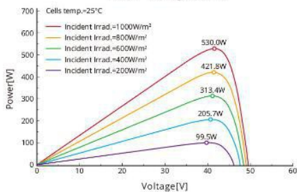
Power-Voltage Curve
