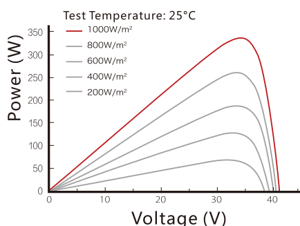
Power curve under different irradiance OLV-335-60M-HB9H
