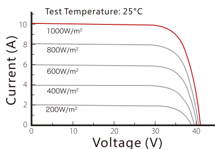
I-V Curves at Different Irradiances OLV-335-60M-HB9H
