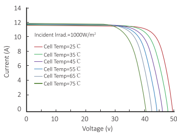
Current-Voltage Curve (SK4-72HPH-440M)
