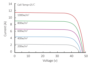
Current-Voltage Curve (SK4-72HPH-440M)
