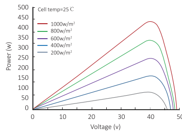
Power-Voltage Curve (SK4-72HPH-440M)
