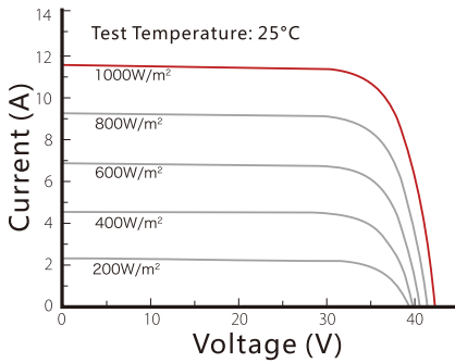
I-V Curves at Different Irradiances OLV-440-72M-HC6H
