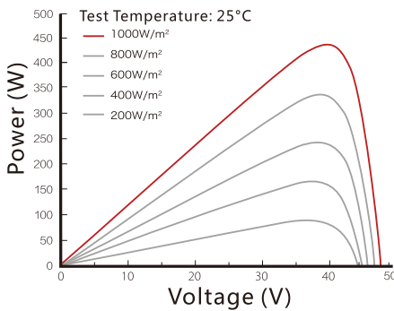
Power curve under different irradiance OLV-440-72M-HC6H
