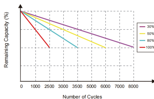
CYCLE LIFE vs. DEPTH OF DISCHARGE(DOD)
