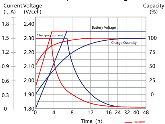
Constant-potential charge
