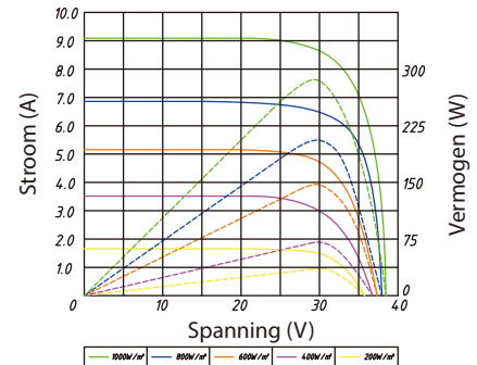
OKM60 Pm(W)290
