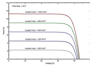
I-V Curve at different irradiation (SPP385QHEH)
