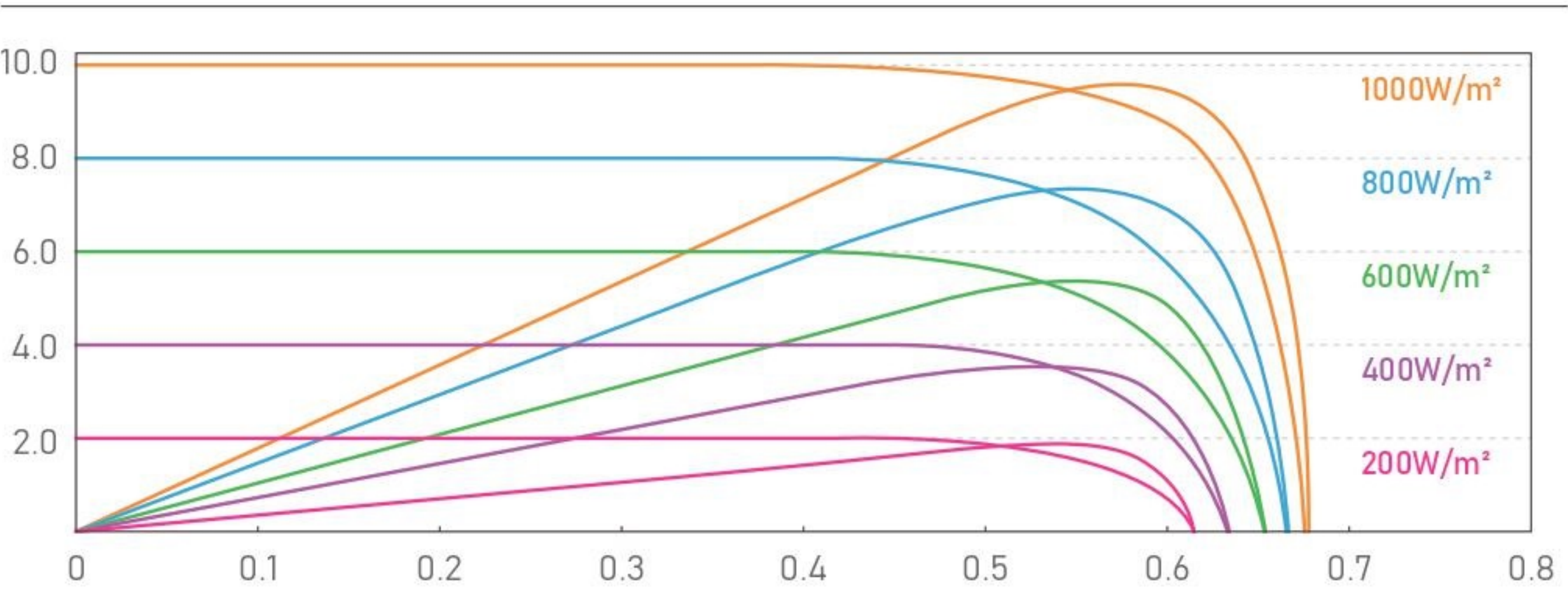
IV Curve
