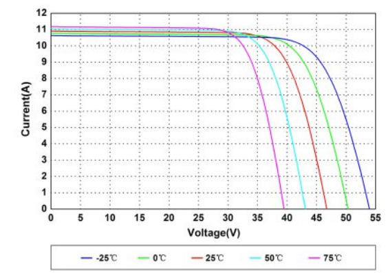
Current-Voltage Curves at Different Temperatures
