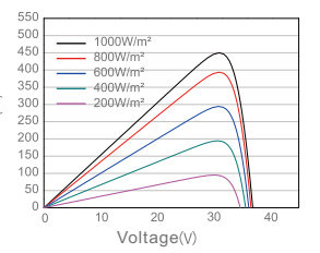
Power Voltage Curve CBG-450M/60
