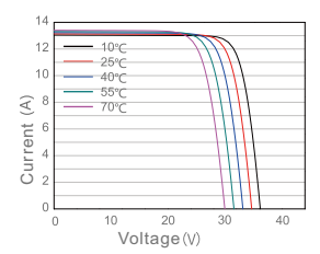
Current Voltage Curve CBG-450M/60
