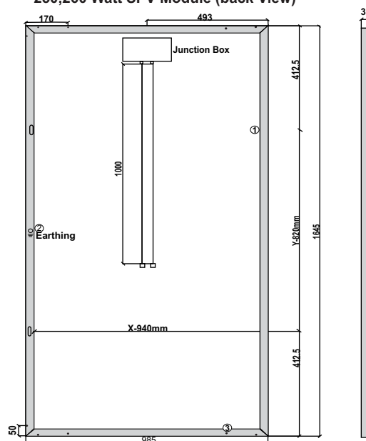
250,260 Watt SPV Module (back View)
