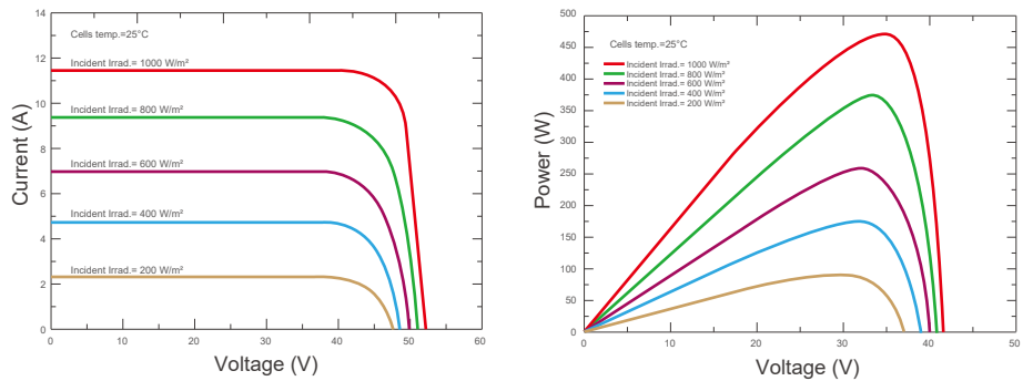
Current-Voltage & Power-Voltage Curves (RMHHB72-470S2)
