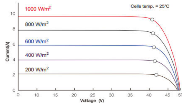
I-V curve
