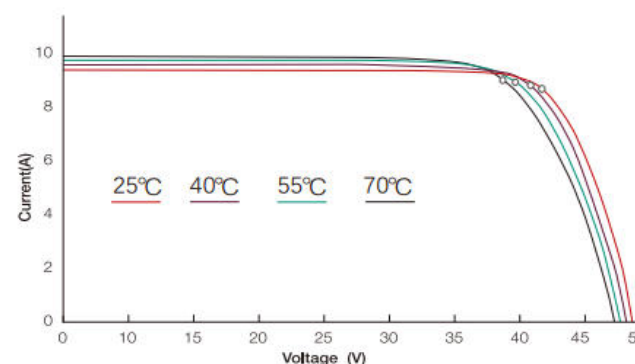
I-V curve
