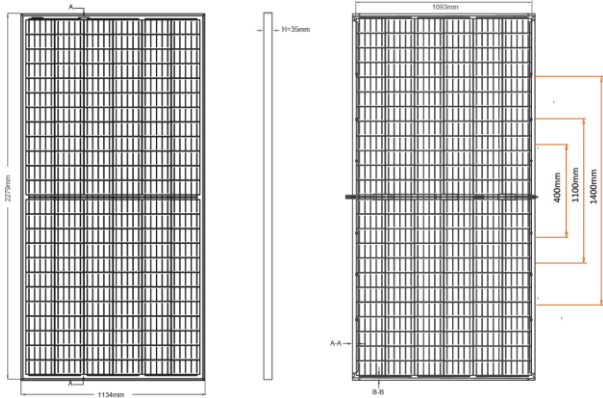
FRONT VIEW SIDE VIEW BACK VIEW Dimensions
