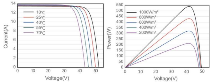
I-V Curves
