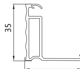
35 Frame Dimension (Unit: mm)
