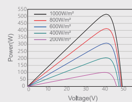
Power-Voltage Curve (500W)
