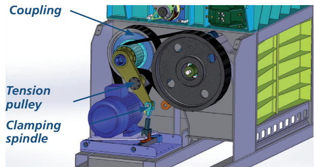
Countershaft gear
