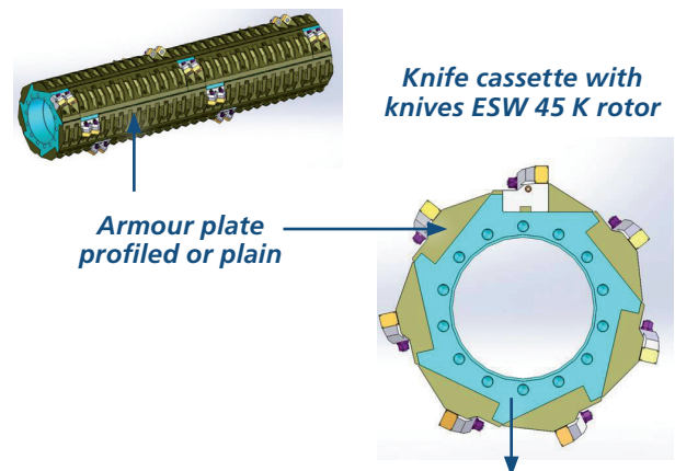
Rotor illustration
