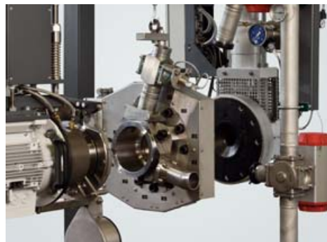
Cutting chamber
