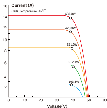
Current-Voltage Curve(SN580-144MT)
