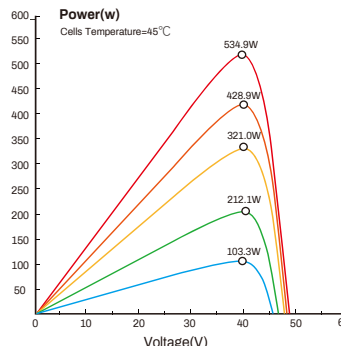
Current-Voltage Curve(SN580-144MT)
