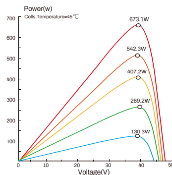
Power-Voltage Curve(SN710-132MTBS)
