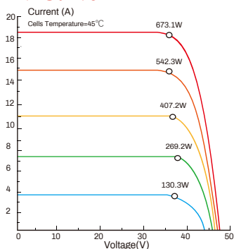
Current-Voltage Curve(SN710-132MTBS)
